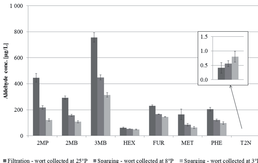
Fig. 3 Extraction of aldehydes during sparging
