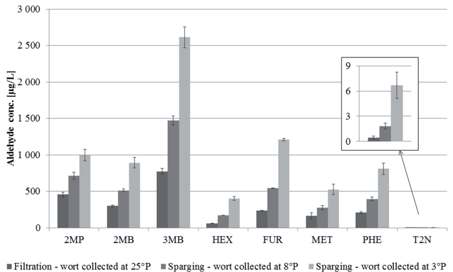
Fig. 4 Extraction of aldehydes during sparging upon extract normalisation to 25 °P
