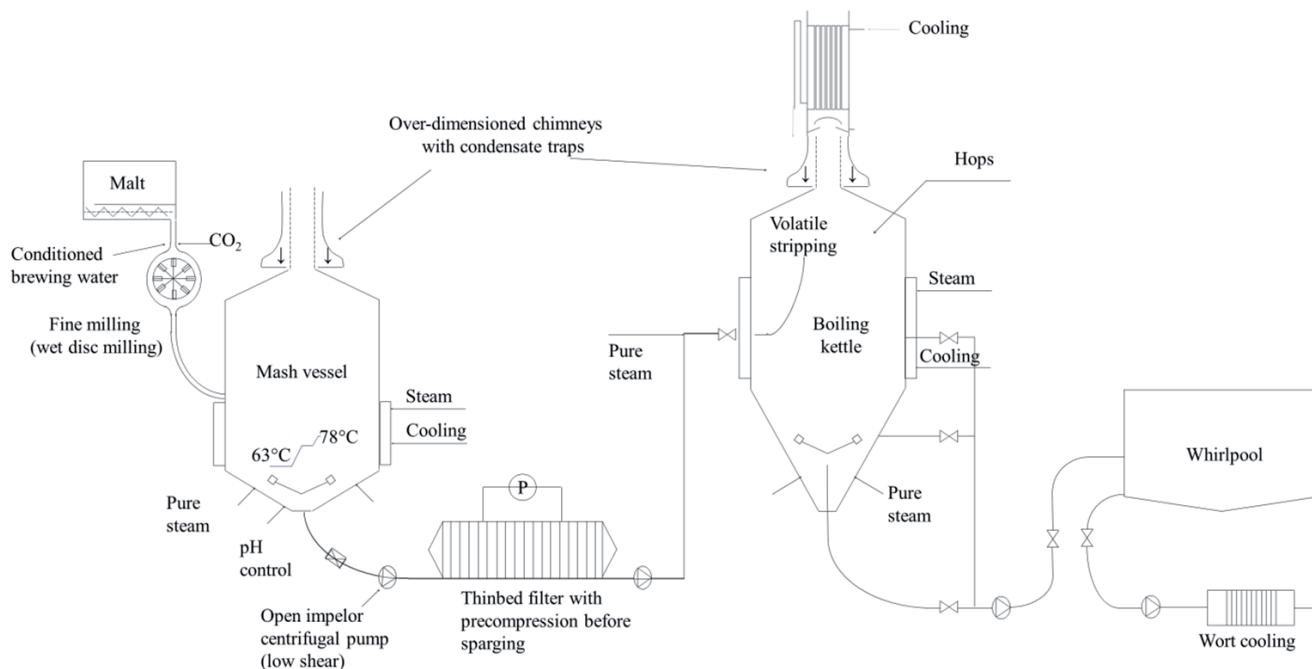
Fig. 1 Scheme of the pilot brewing plant
