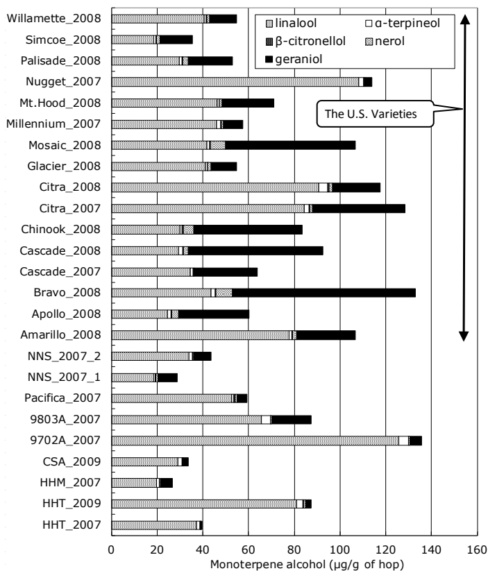
Fig. 2 Composition of monoterpene alcohols (µg/g of hop) in various hops : HHT, Hallertauer Tradition; HHM, Hallertauer Magnum; CSA, Czech Saaz; NNS, New Zealand Nelson Sauvín. (This figure was previously shown in ref. 49)
