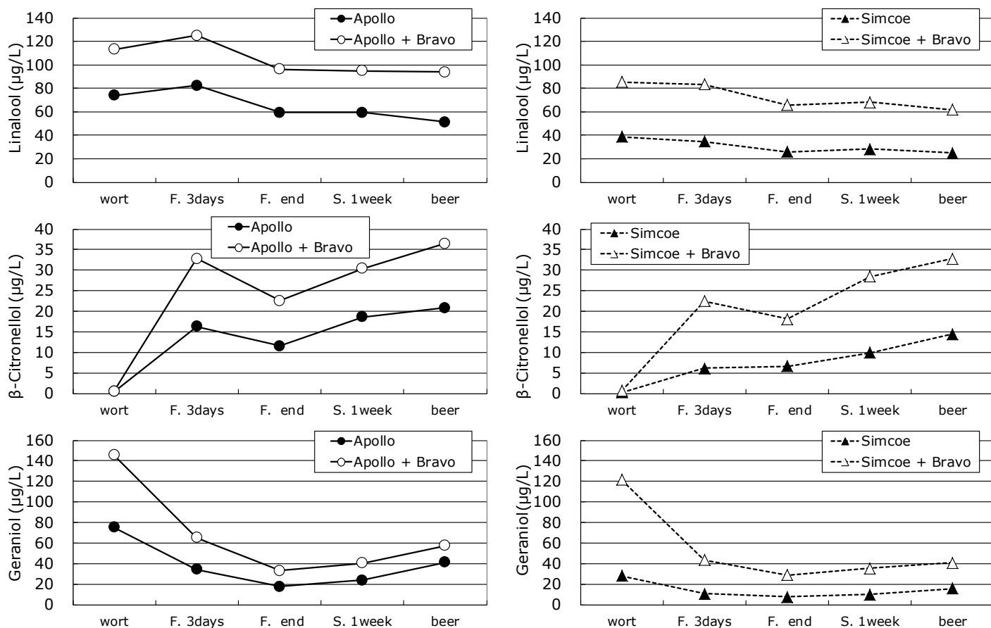
Fig. 4 Comparison of monoterpene alcohols (µg/L) during fermentation with blend-hopping: F., fermentation; S., Storage; Flavouring hop dosage; ● Apollo (Apollo 0.8 g/L); ○ Apollo + Bravo (Apollo 0.8 g/L + Bravo 0.4 g/L); ▲ Simcoe (Simcoe 0.8 g/L); △ Simcoe + Bravo (Simcoe 0.8 g/L + Bravo 0.4 g/L)
