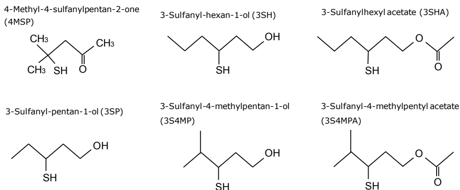
Fig. 3 Major volatile thiols derived from hops (On the basis of ref. 4, 13–14, 22–23, 26–27, 39–40, 43–46)
