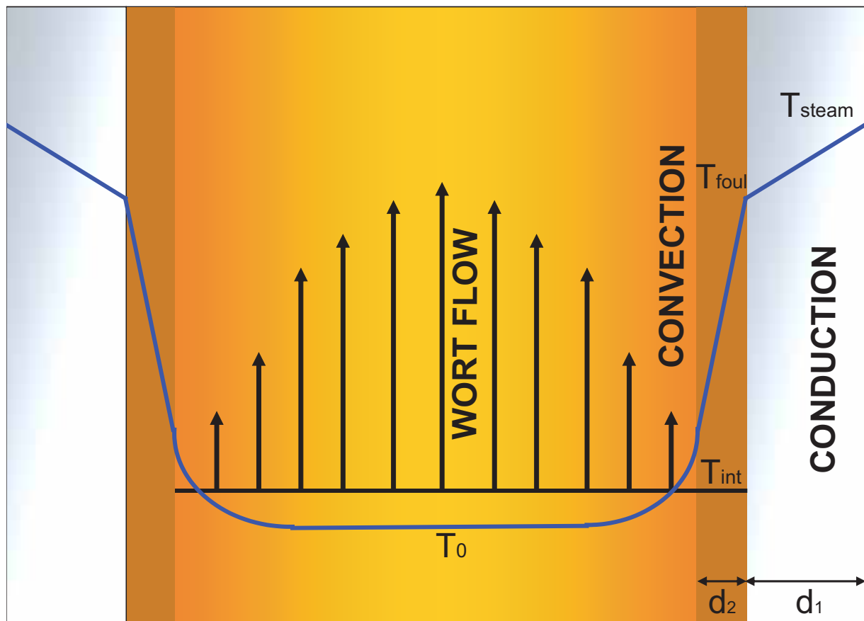
Figure 11 Heat transfer by conduction and convection in a boiling system, with an additional conduction/insulation due to fouling ( T_{steam} = temperature at the outlet of steam unit; T_{foul} = temperature at the interface wall/fouling layer; T_{int} = temperature at the interface wort/fouling layer; T_0 = boiling temperature of the wort)
