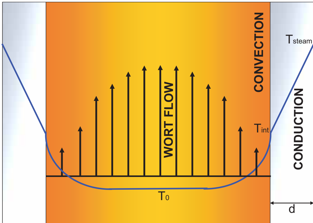
Figure 10 Heat transfer by conduction and convection in a boiling system ( T_{\text{steam}} = temperature at the outlet of steam unit; T_{\text{int}} = temperature at the interface wort/wall; T_0 = boiling temperature of the wort)
