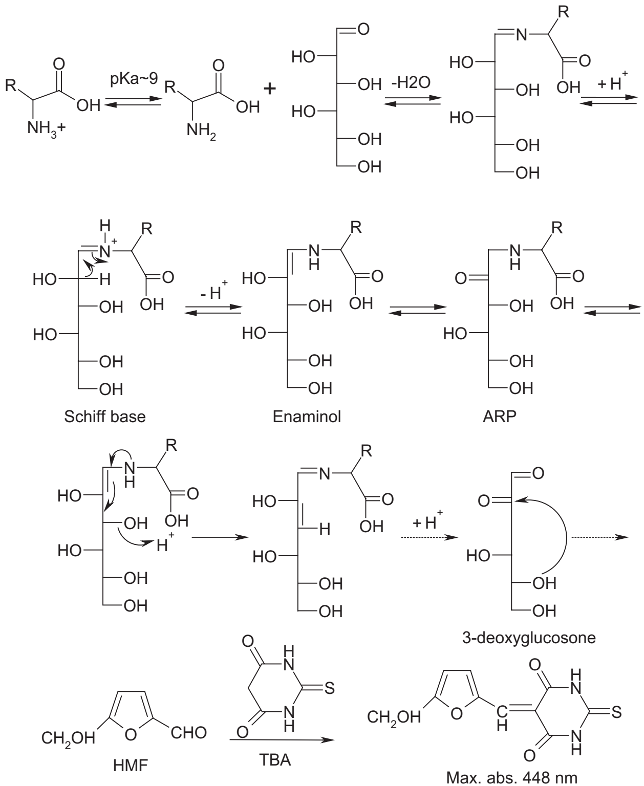
Figure 1 Maillard reaction leading to the formation of HMF and the subsequent reaction with TBA (ARP:Amadori Rearrangement Product; HMF: 5-hydroxymethylfurfural)
