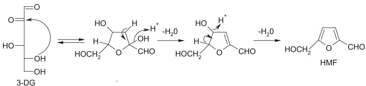
Figure 4 Detail of the cyclization of 3-DG and subsequent dehydration reactions leading to HMF
