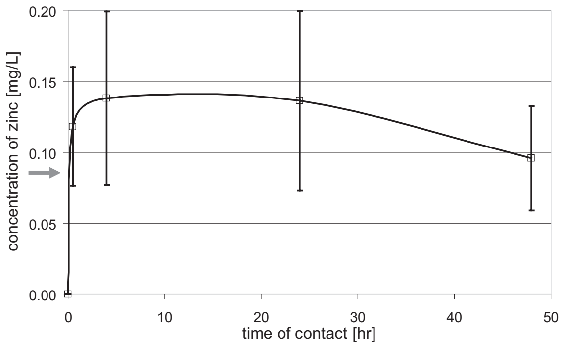
Fig. 6: Release of zinc after addition of hot trub to wort (800 mg /L (d.m.) at t = 0 ) vs. contact time of trub and wort ( n = 6 , p = 0.95 ). The arrow indicates the original content in wort prior to yeast treatment, while the origin of the diagram ( t = 0 ) represents the value after yeast treatment right before trub addition. For each trial the zinc concentration at t = 0 was set to "0" and all other values relate to this set point
