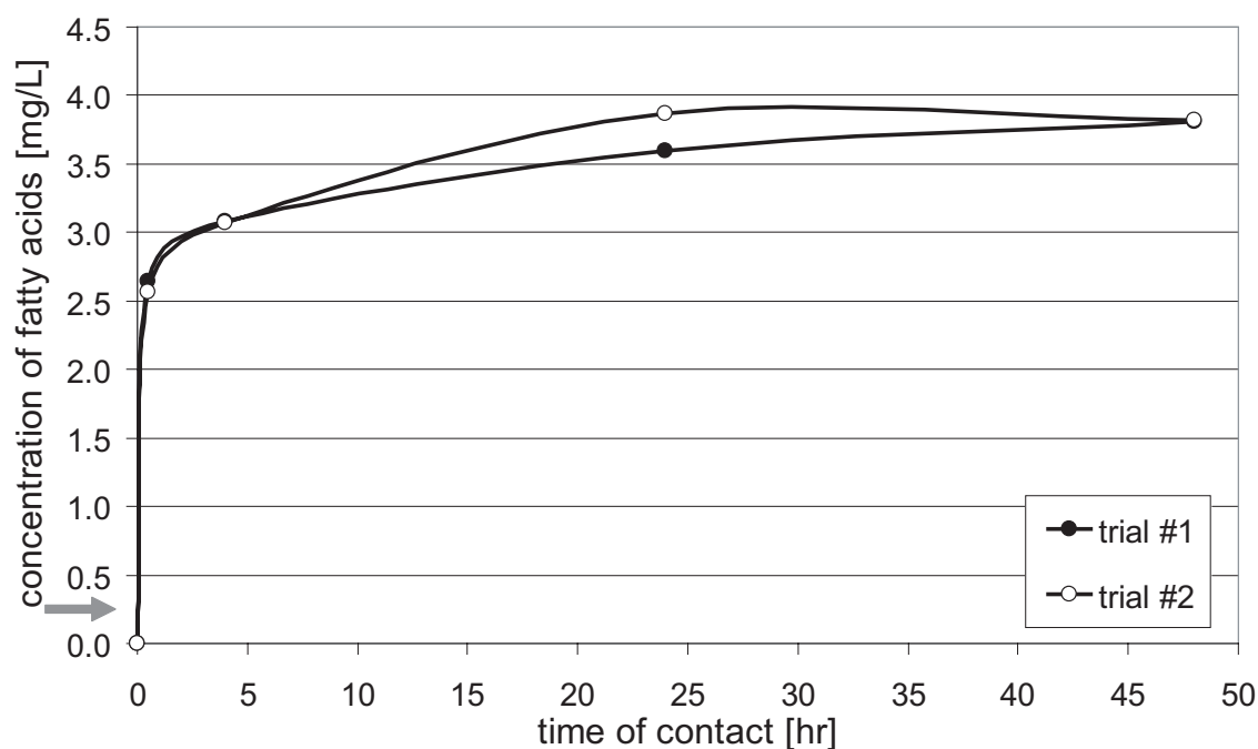
Fig. 4: Long-chain fatty acids (C14-C18:3) in suspension after addition of hot trub to wort (800 mg /L (d.m.) at t = 0 ; no separation of trub particles) vs. contact time of trub and wort. The arrow indicates the original content in wort prior to yeast treatment, while the origin of the diagram ( t = 0 ) represents the value after yeast treatment right before trub addition. For each trial the fatty acid concentration at t = 0 was set to "0" and all other values relate to this set point.
